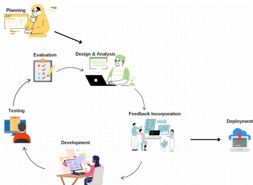
Figure 1: Iterative process
